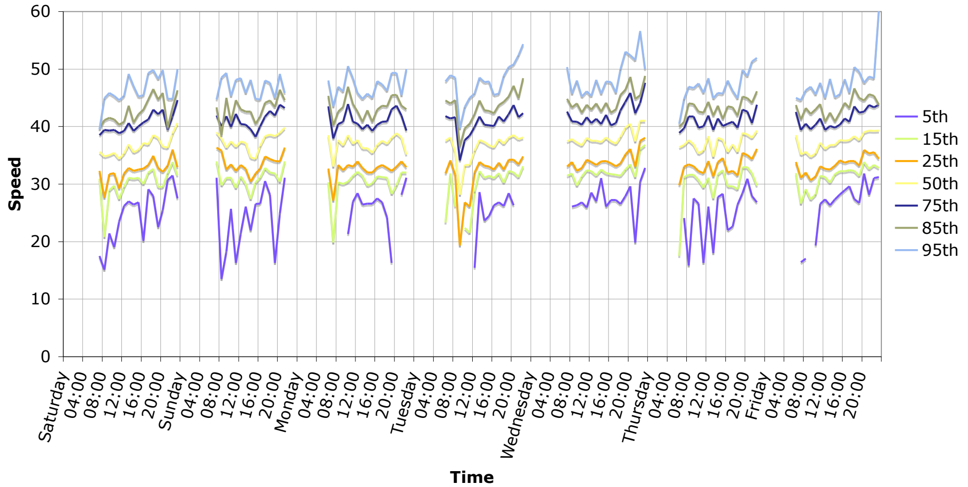
Percentiles of per-hour speed distributions by hour over a week (Northwest bound / leaving village)
