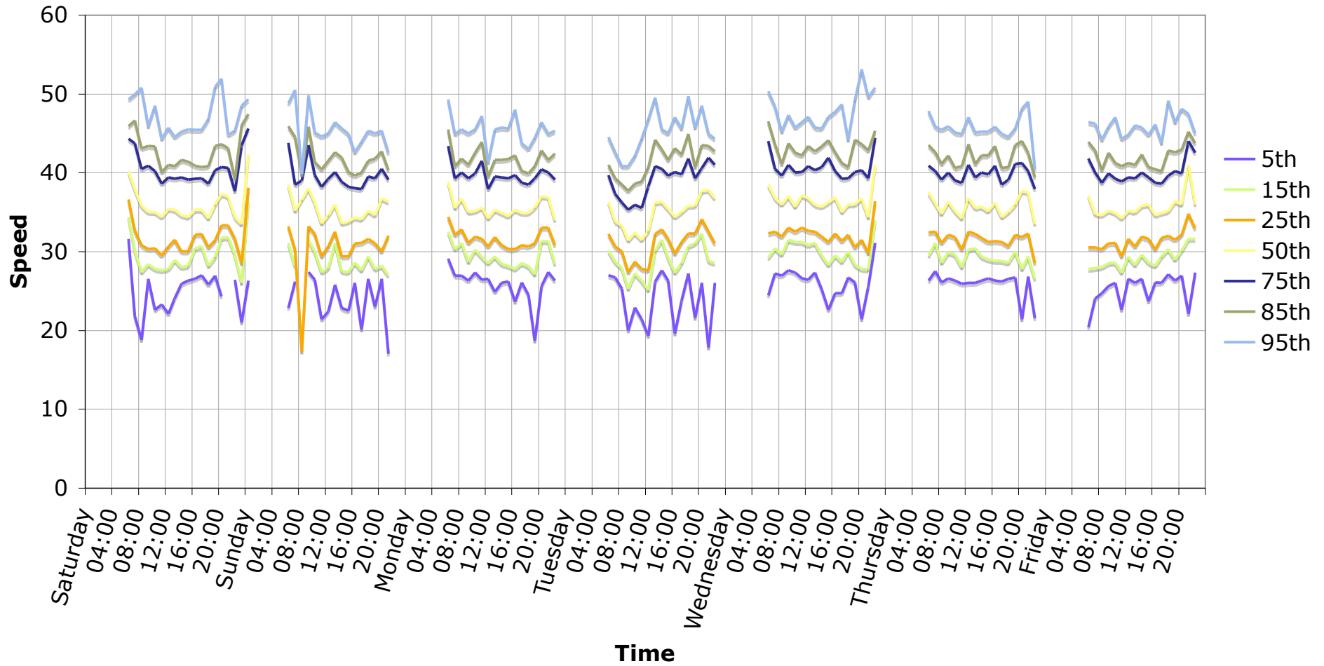
Percentiles of per-hour speed distributions by hour over one week (Southeast bound / entering village)
