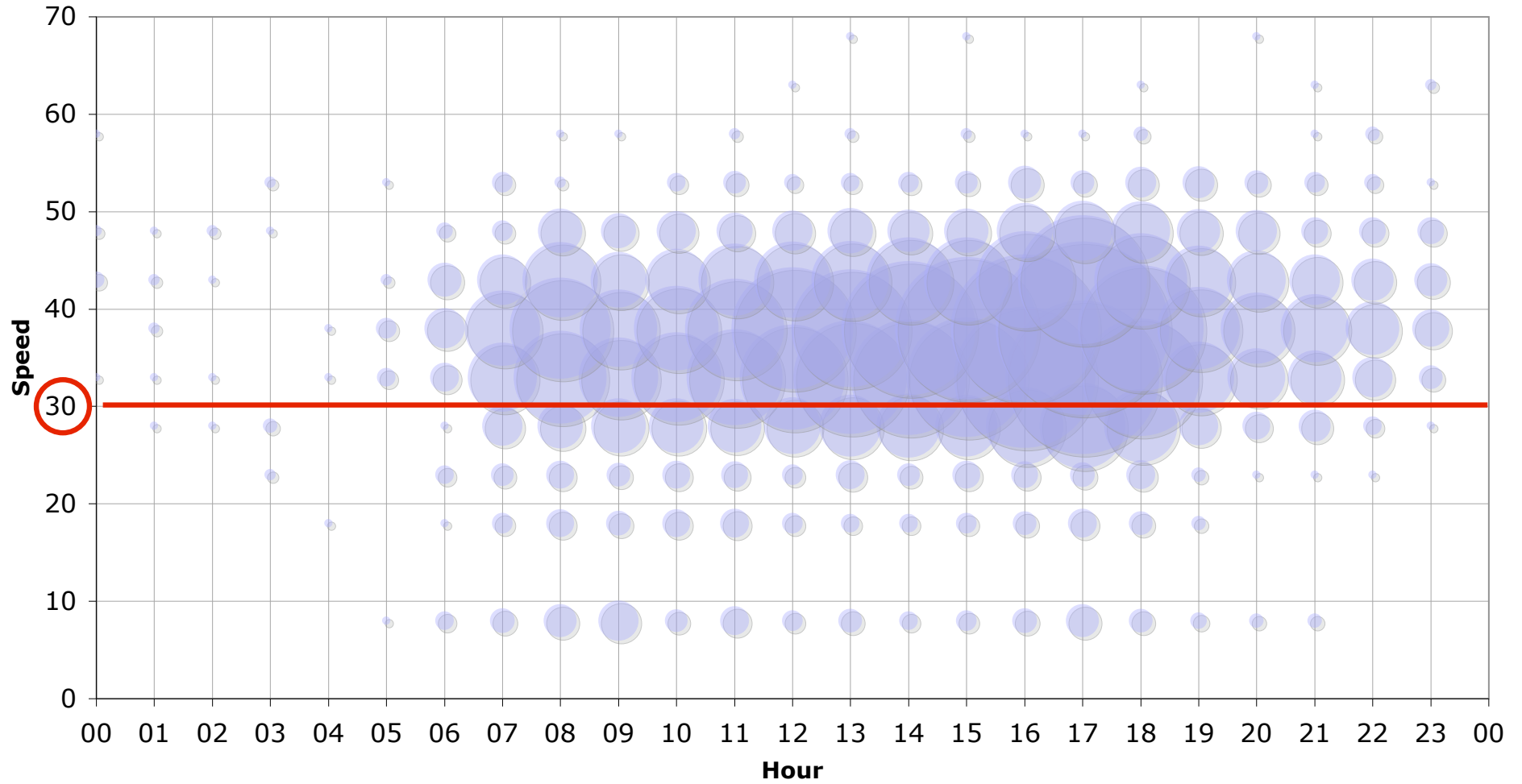
Number of vehicles by speed and time of day Northwest bound, Weekdays 25th-29th February 2008
